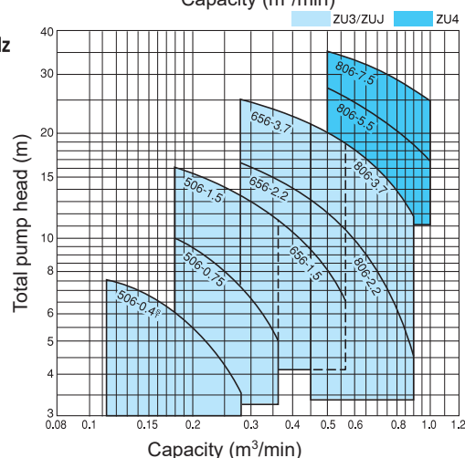
ZU4 type (Pedestal support type) Floor mount is also available.
