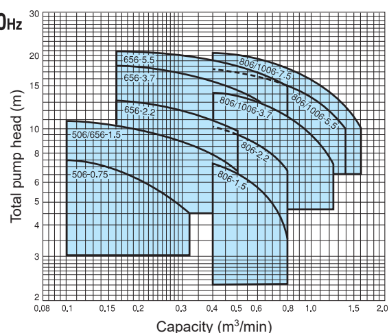
AU4 type (Pedestal support type)
