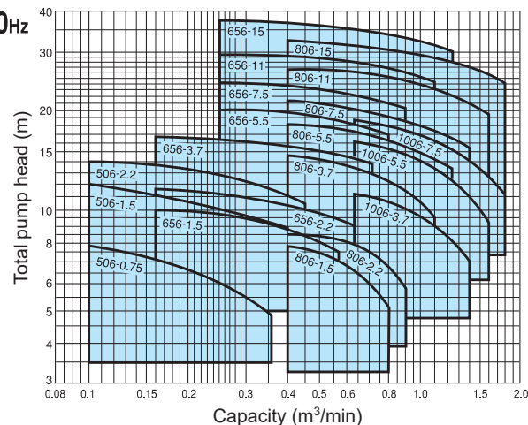
VU4 type (Pedestal support type)
