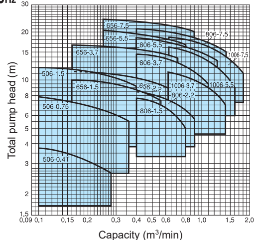
VUS type (Pedestal support type) Note: Guide pipes are not included.
